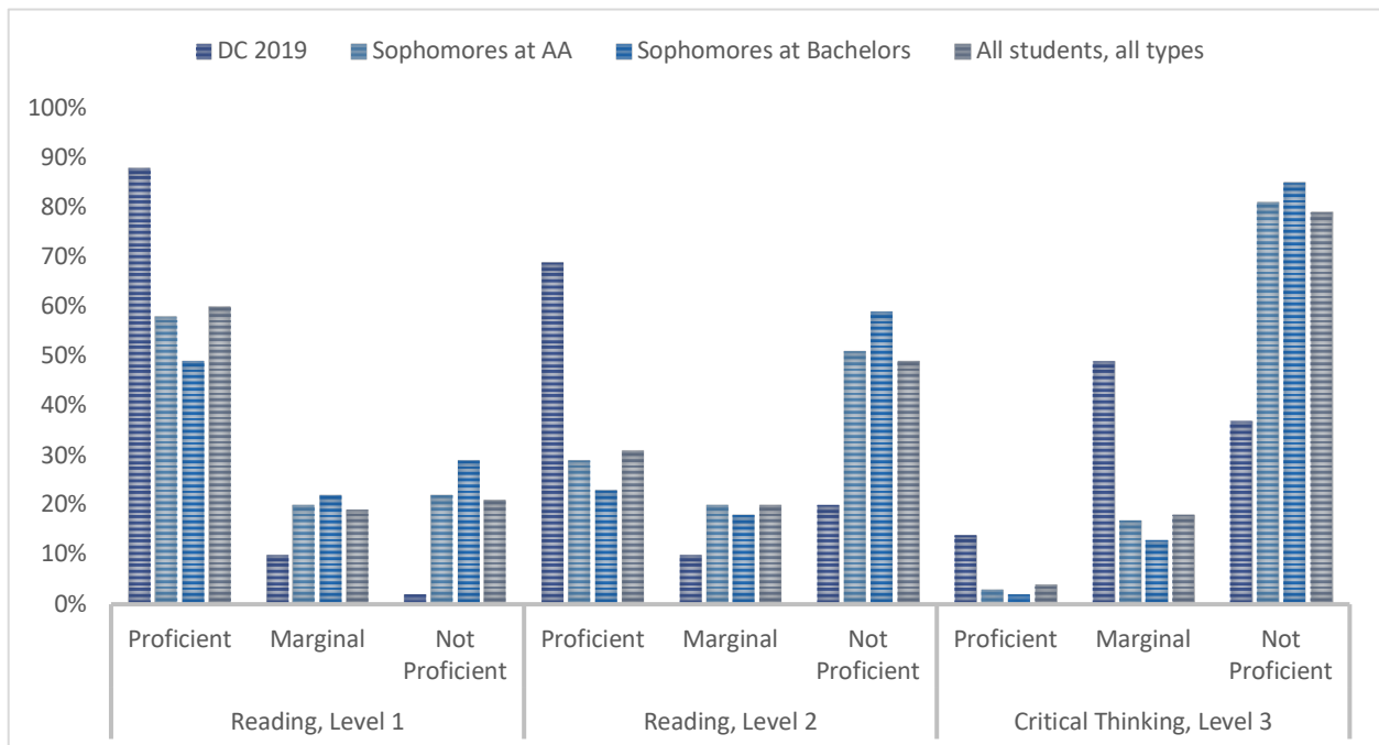
Figure 3: Proficiency Classification Comparison—Reading and Critical Thinking
