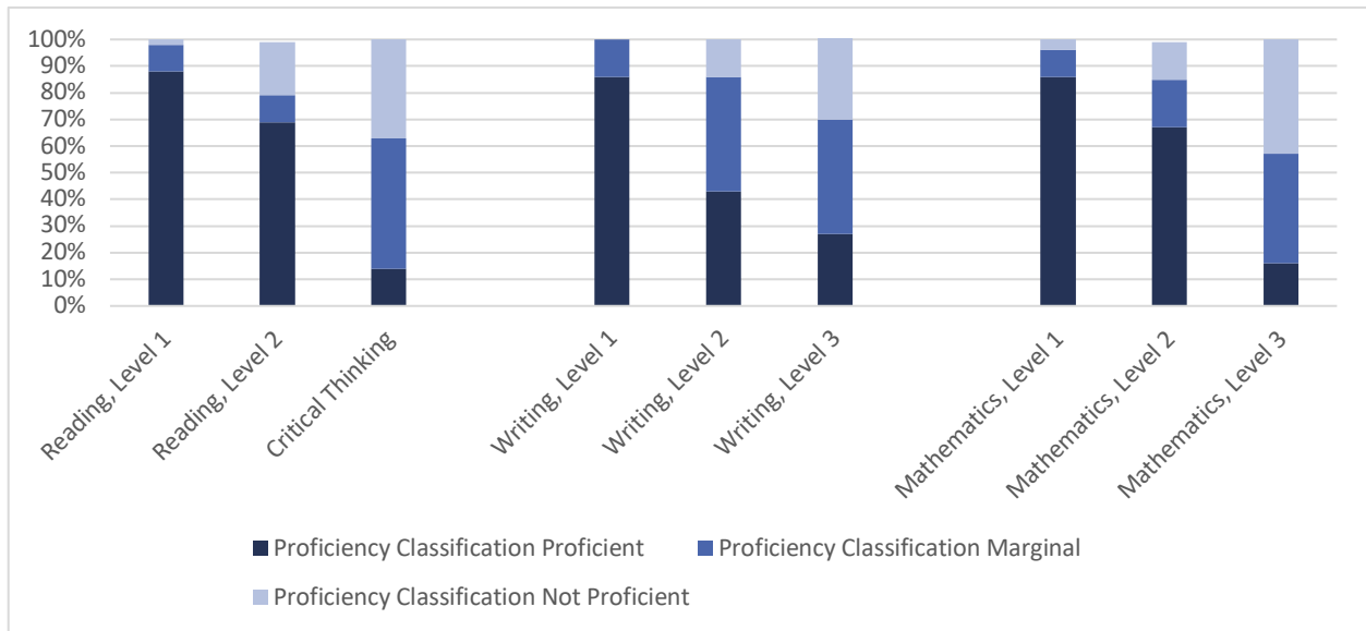
Figure 2: Proficiency Classification Estimates Graph—DC Class of 2019
