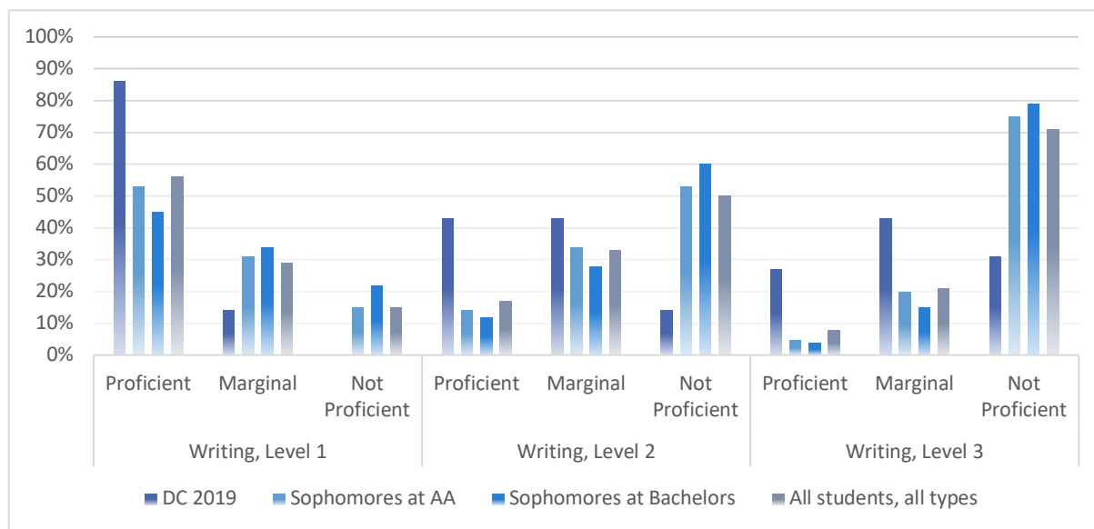
Figure 4: Proficiency Classification Comparison—Writing
