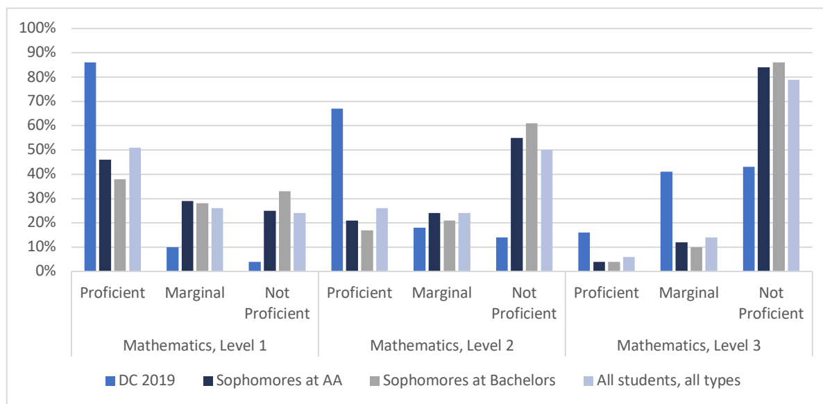
Figure 5: Proficiency Classification Comparison—Mathematics
